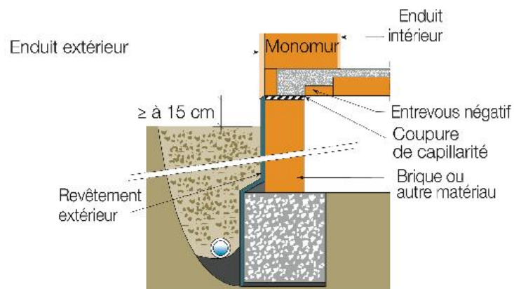
Figure 16. Water barrier.
