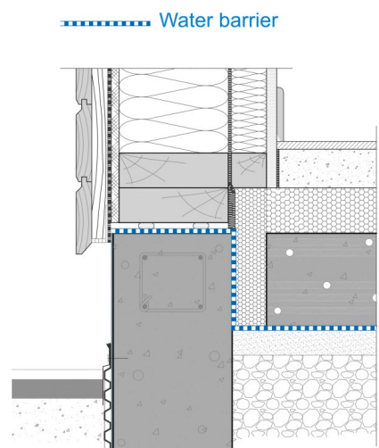
Figure 16. Water barrier.
