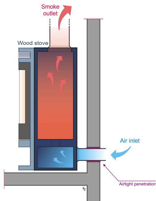
Figure 19. Airtight wood stove with outside air intake.
